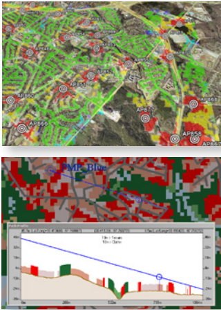
Top Image: Mesh Network Design showing Coverage Heatmap Bottom Image: Dynamic Path Profiler showing terrain and clutter heights
